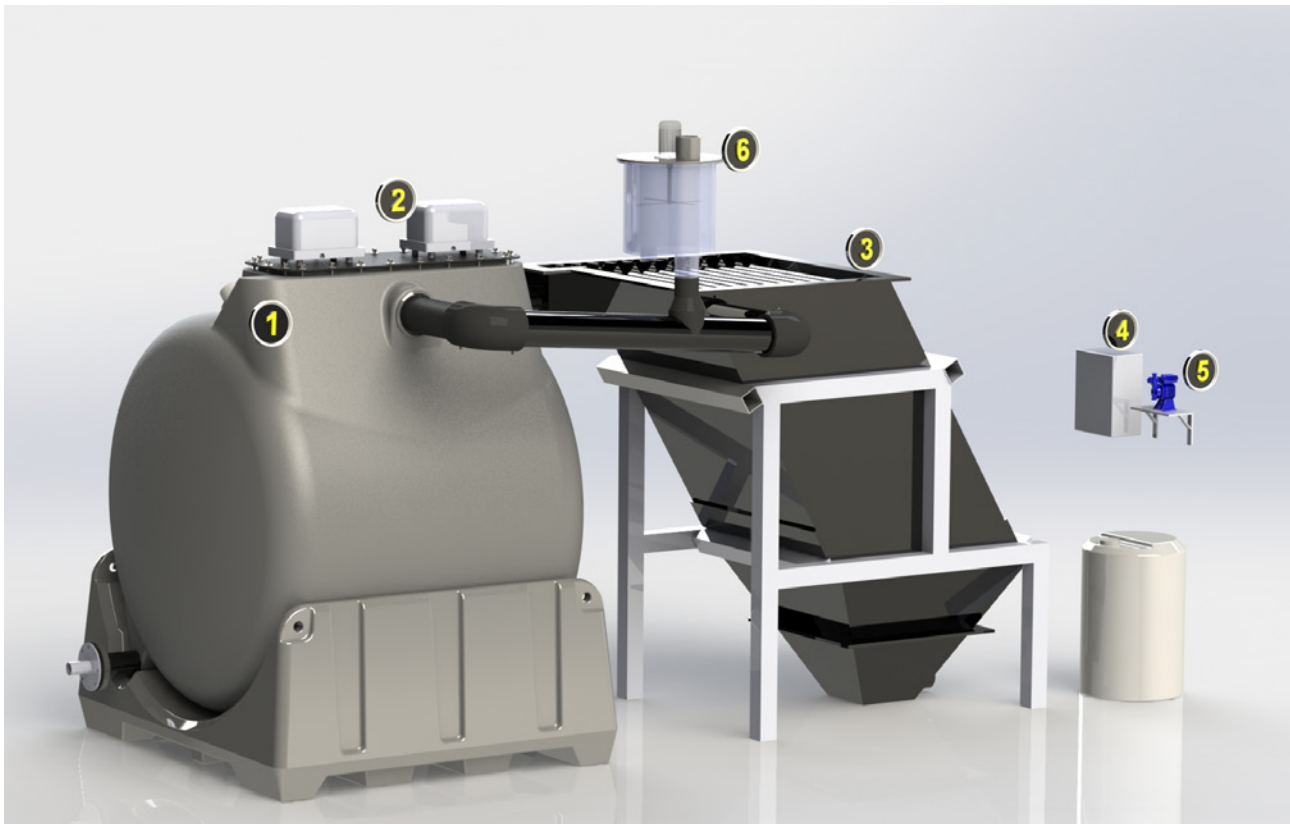
1. Biological filter 2. Aeration 3. Solid-liquid separation 4. Automation 5. Nutrient dosing 6. Excess foam breaking
